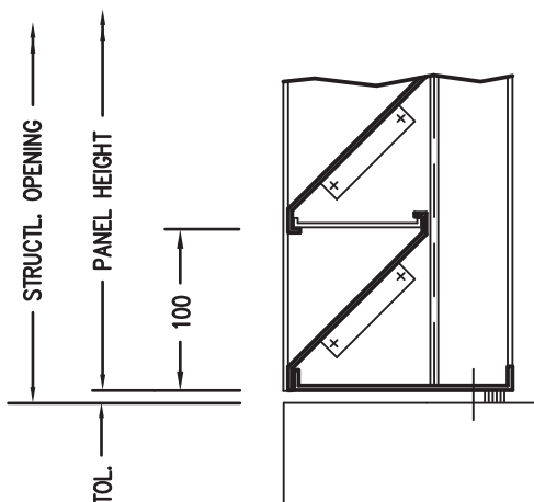
708. 100 BLADE CILL DETAIL
