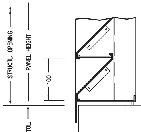
701. 100 BLADE CILL DETAIL
