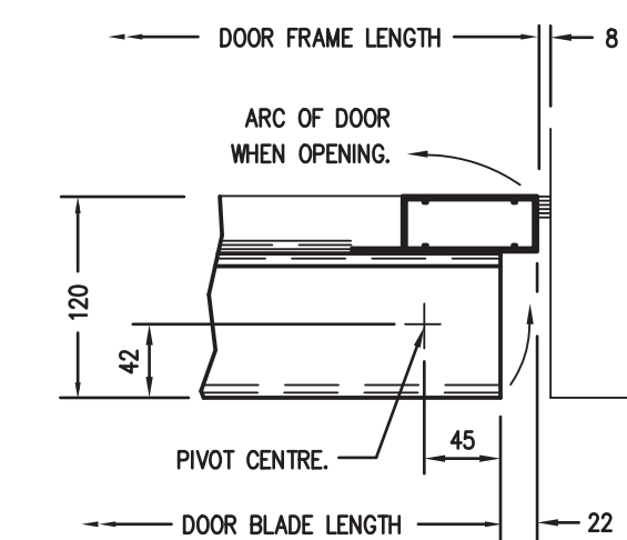
725. R/H D FRAME INTO STRUCTURE
