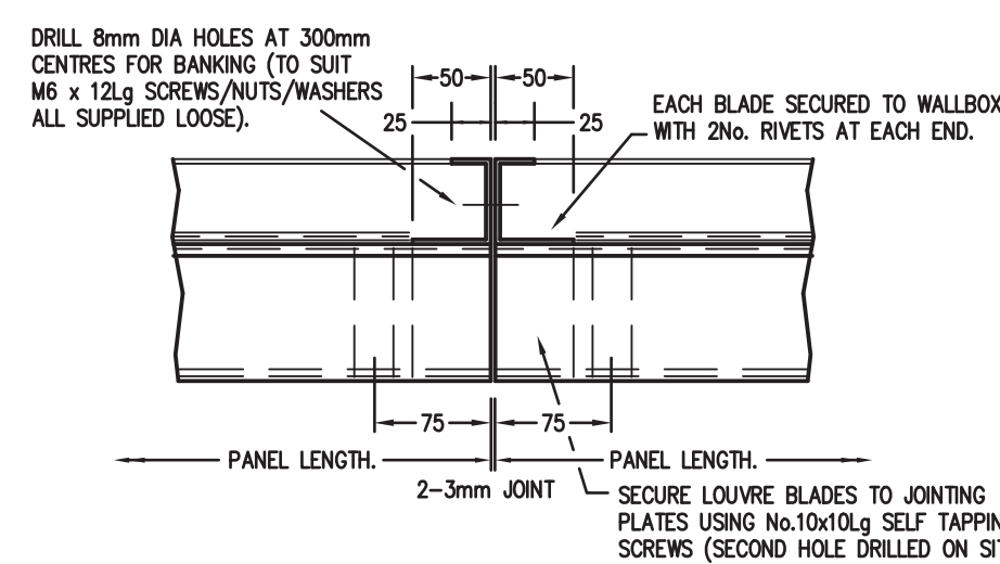
703. HORIZONTAL JOINT DETAIL
