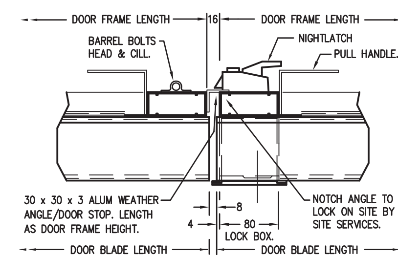
724. MEETING LOCK STILES
