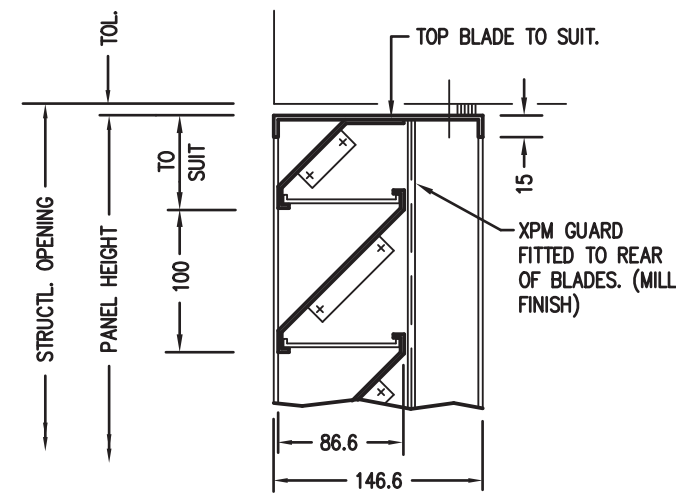
707. HEAD DETAIL
