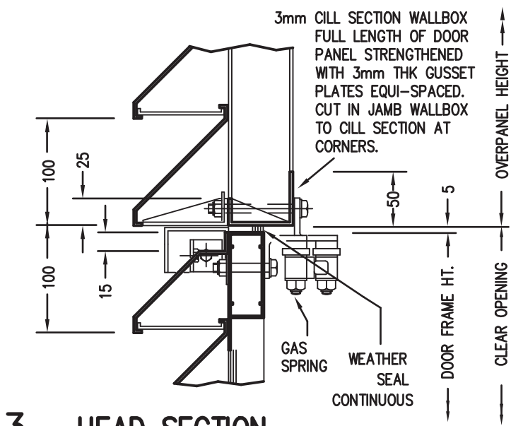
723. HEAD SECTION
