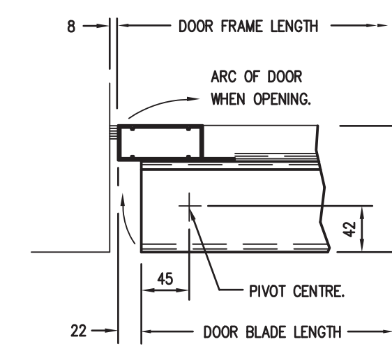
726. L/H D FRAME INTO STRUCTURE
