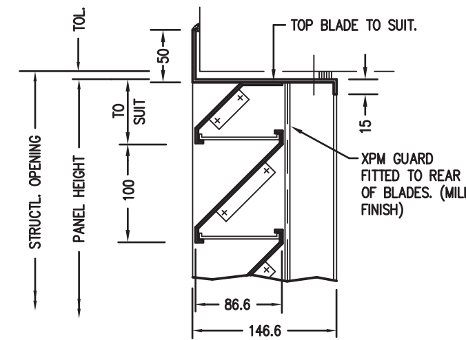
700. HEAD DETAIL
